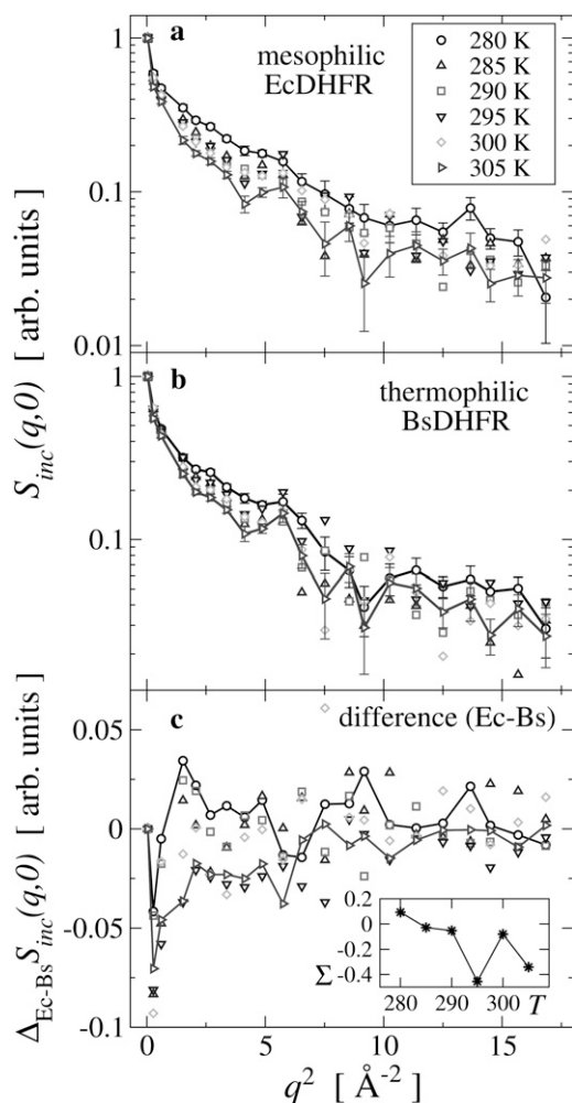
FIGURE 2 Elastic scattering intensity, S_{inc}(q, 0) measured at various temperatures for (a) Ec DHFR and (b) Bs DHFR. For clarity, representative error bars are shown only for the 280 K and 305 K data. Connecting lines are drawn for convenience and the vertical axes are logarithmic. (c) The difference, \Delta_{Ec-Bs} S_{inc}(q, 0) = S_{inc}^{Ec}(q, 0) - S_{inc}^{Bs}(q, 0) , for each temperature; the inset shows the integrated difference, \Sigma(T) = \sum_q \Delta_{Ec-Bs} S_{inc}(q, 0) plotted against temperature, T .
